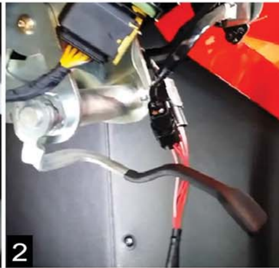
2 Attach Keyless Ignition Power Harness mating connectors to both ends of Ignition Switch connector
