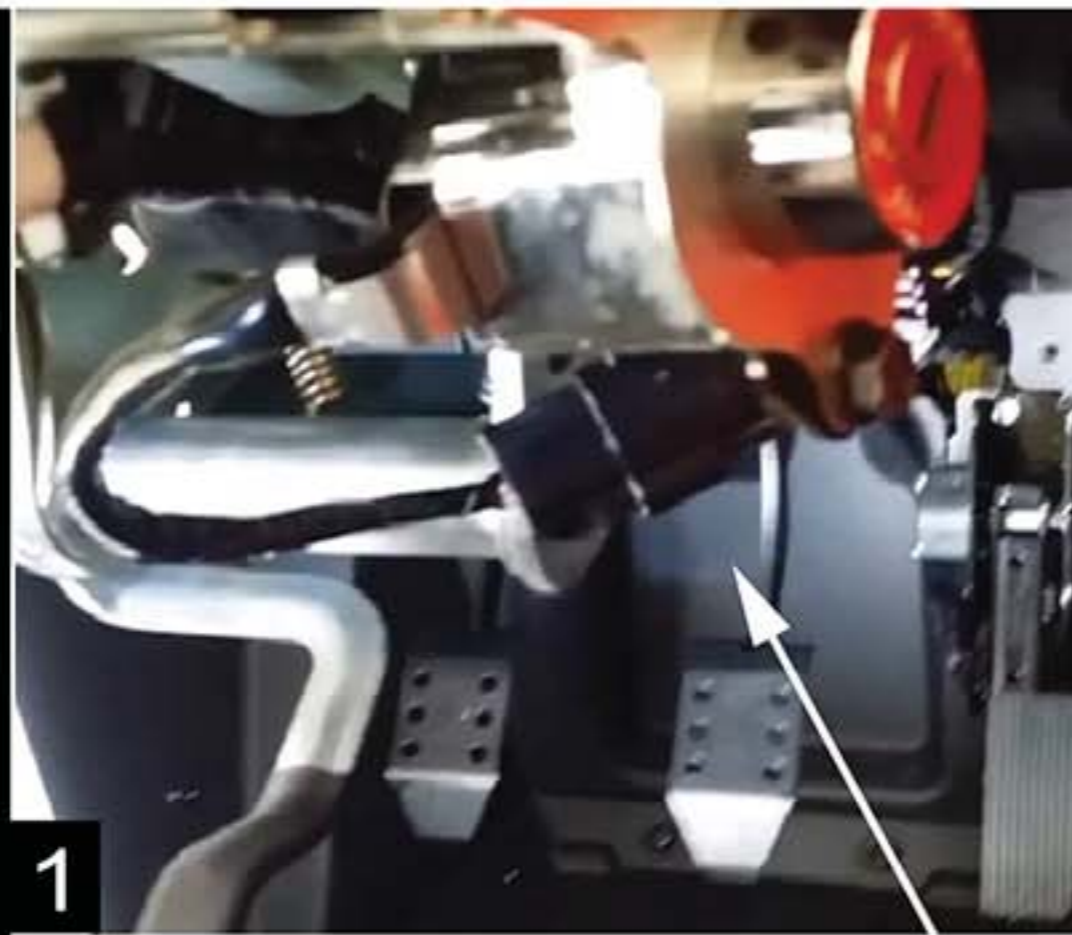
1 Remove lower dash panel and locate Ignition Switch Connector. Separate Connector ends.
